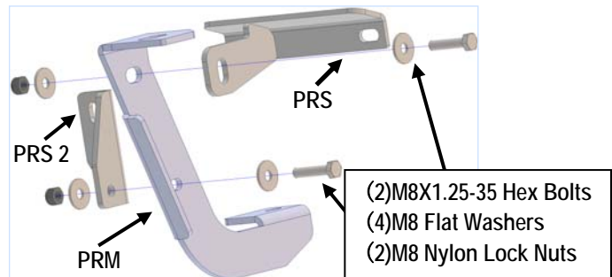
(Fig 4) Passenger Rear Mounting Bracket Assembly
