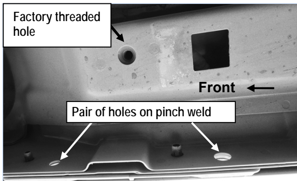
(Fig 2) Passenger Side Front Mounting Location
