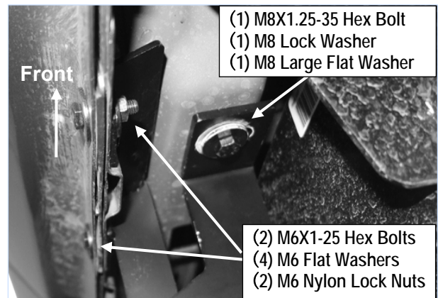
(Fig 3) Passenger Front Mounting Bracket Installed
