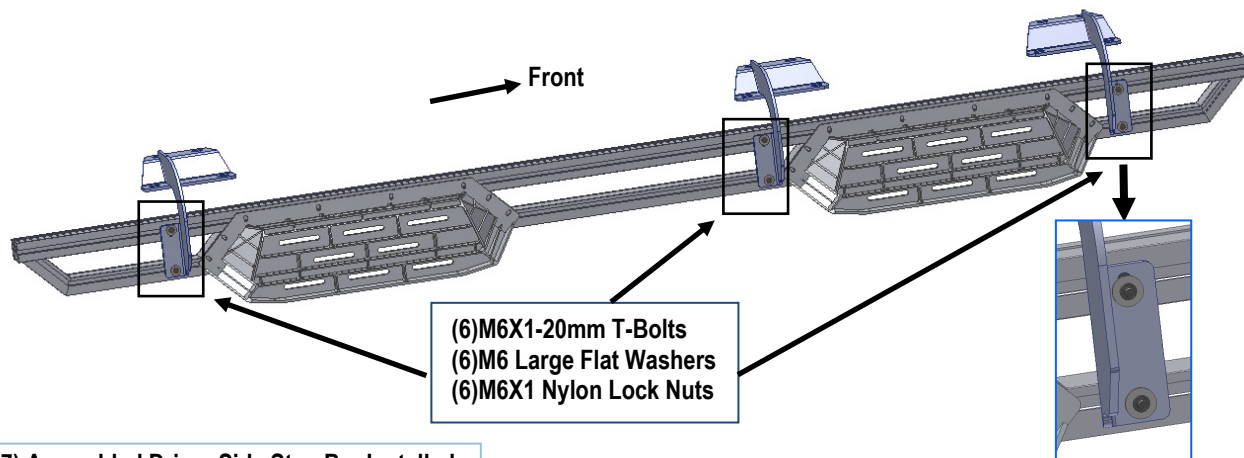
(Fig 7) Assembled Driver Side Step Bar Installed
