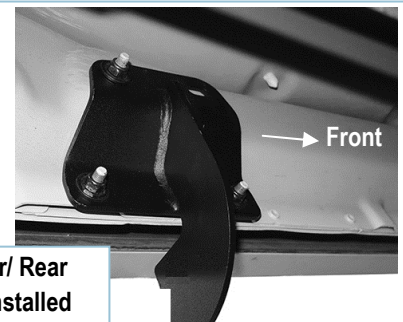
(Fig 5) Driver Center/ Rear Mounting Bracket Installed
