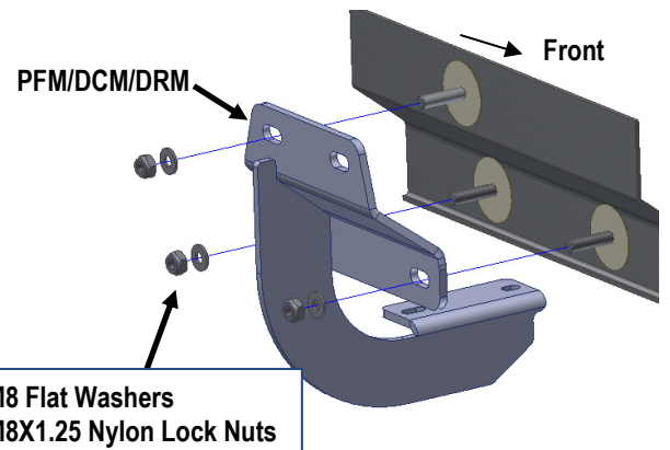
(Fig 5) Driver Center/ Rear Mounting Bracket Installed
