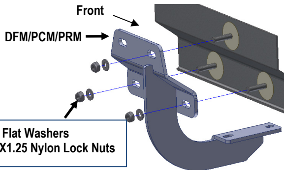
(Fig 3) Driver Front Mounting Bracket Installed
