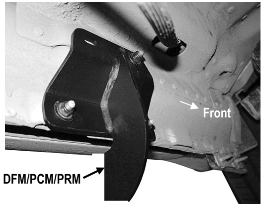
(Fig 4) Driver Front Mounting Bracket Installed
