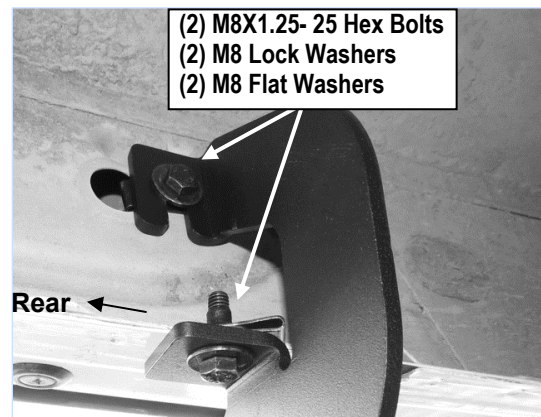
(Fig 8) Driver Center Mounting Bracket (DCM) Installed
