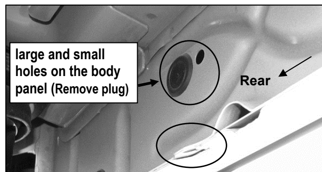
(Fig 4) Flat tab on Pinch Weld with hole (Driver Side Rear Mounting Location)
