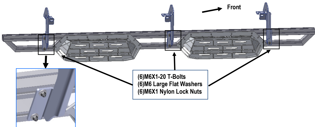
(Fig 9) Assembled Driver Side step Bar Installed
