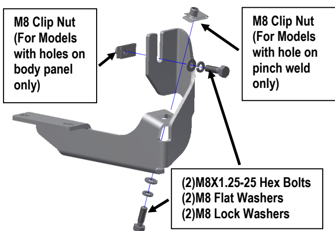
(Fig 13) Passenger Front Mounting Bracket (PFM) Installed
