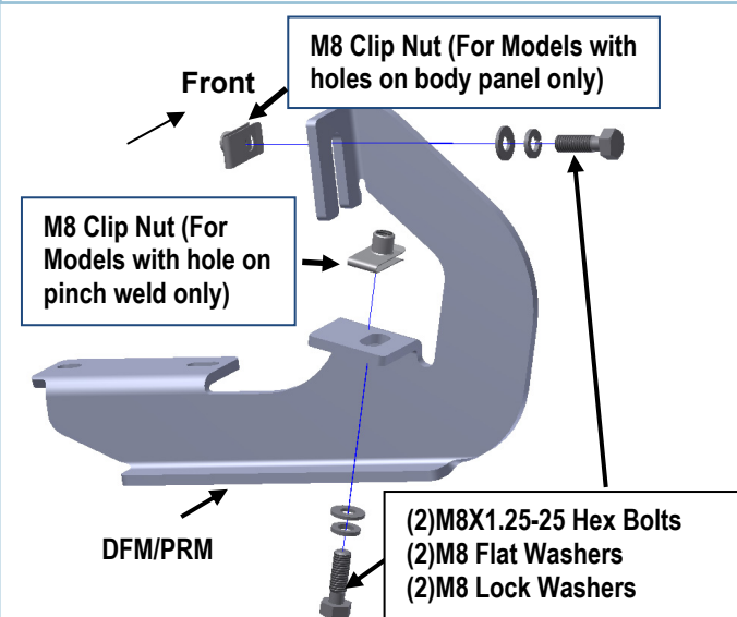
(Fig 6) Driver Front Mounting Bracket (DFM/PRM) Installed
