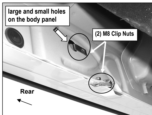
(Fig 5) Flat tab on Pinch Weld with hole (Driver Side Rear Mounting Location)
