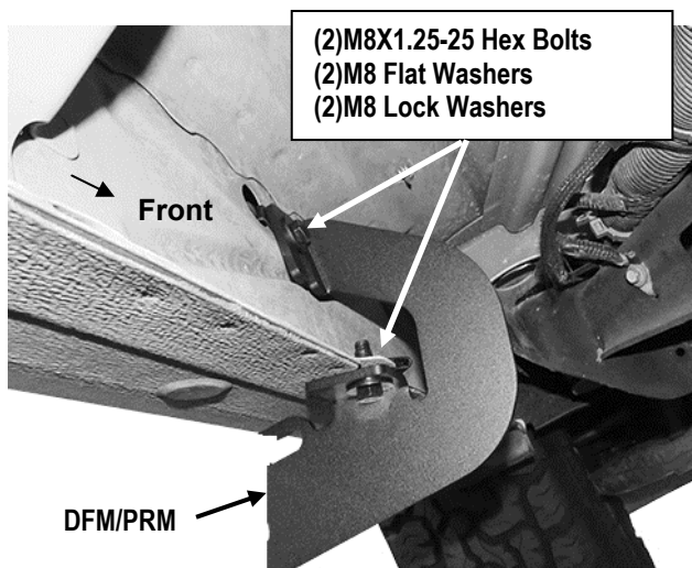
(Fig 7) Driver Front Mounting Bracket (DFM/PRM) Installed
