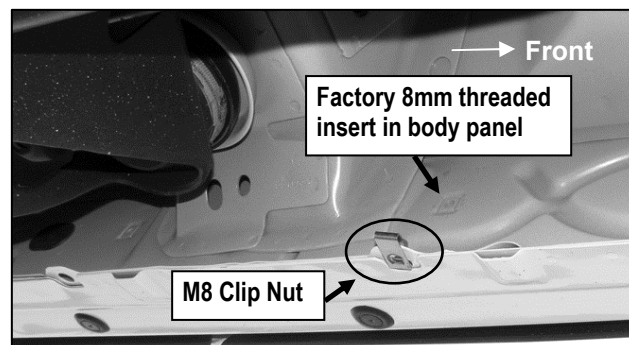
(Fig 3) Flat tab on Pinch Weld with hole (Driver Side Center Mounting Location)
