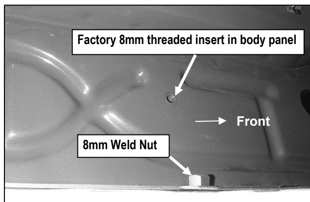
(Fig 2) Flat tab on Pinch Weld with Factory Installed Weld Nut (Passenger Side Front Mounting Location)
