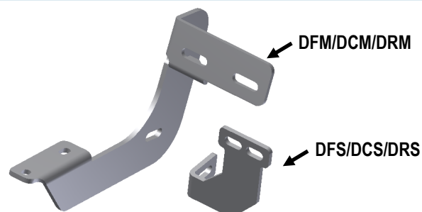
(Fig 6) Driver Front Mounting Bracket
