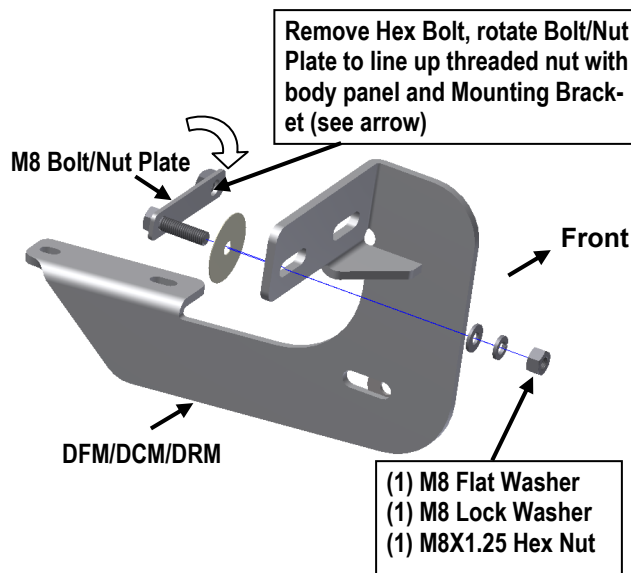
(Fig 7A) Attach Driver Front Mounting Bracket to M8 Bolt/Nut Plate
