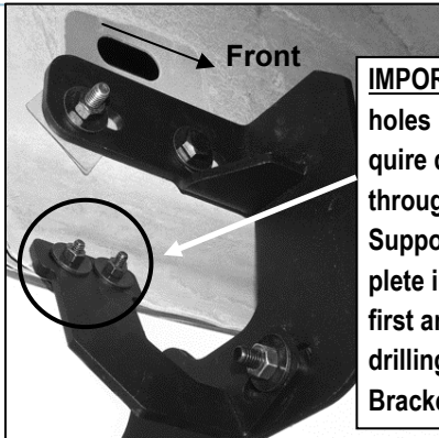
(Fig 12) Driver Front Brackets installed
