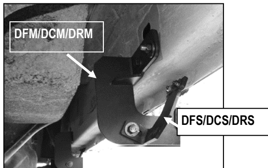
(Fig 14) Driver Center Brackets installed
