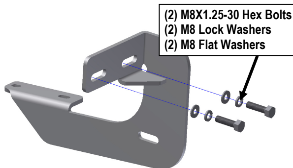
(Fig 9) Driver Front Mounting Bracket for models w/ factory installed threaded inserts (M8 Bolt/Nut Plate not required)
