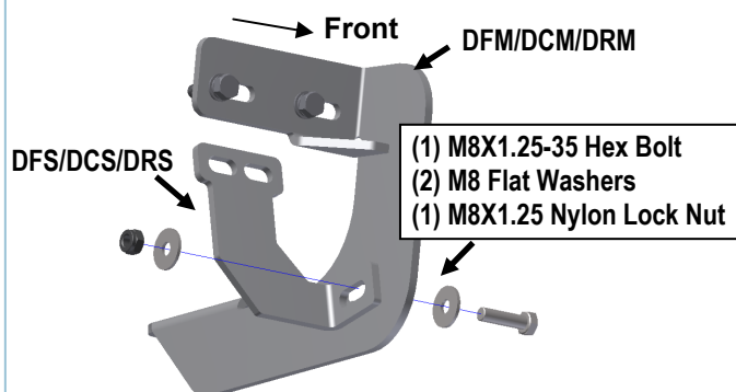
(Fig 10) Attach Driver Front Support Bracket to Drive Front Mounting Bracket
