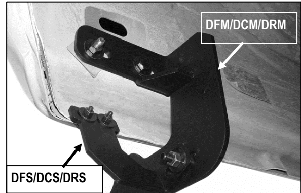
(Fig 16) Driver Rear Brackets installed
