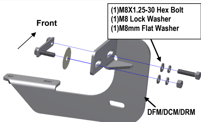
(Fig 7B) Attach Driver Front Mounting Bracket to threaded end of the M8 Bolt/Nut Plate
