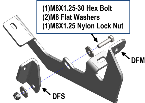
(Fig 2) Driver Front Mounting Bracket Assembly
