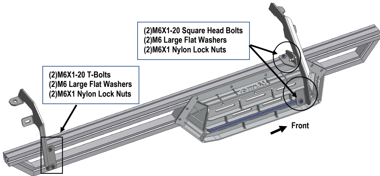
(Fig 6) Assembled Driver Side step Bar Installed
