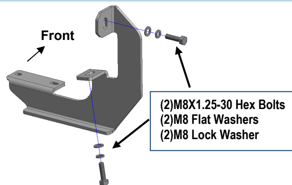
(Fig 5) Driver Rear Mounting Bracket Installed
