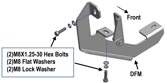
(Fig 3) Driver Front Mounting Bracket Installed
